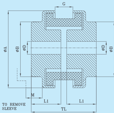
FLANGE TYPE-'S'
