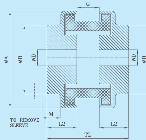
FLANGE TYPE-'J'
